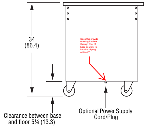
End View
